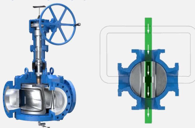
NEUTRAL FULLY UNSEATED – MID TRAVEL
