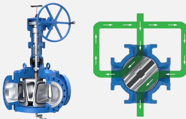
SEATED IN L/R OPEN – CW POSITION
